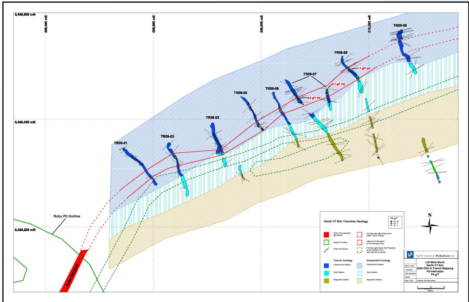
Figure 9. Geological map showing the locations of the 2009 trenches on the North Pit-NVT Rim area, Lac des Iles mine.
