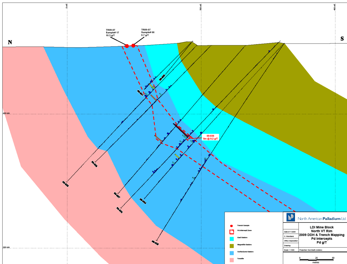
Figure 8. Interpreted geological cross section with assay results for the North Pit-NVT Rim area, Lac des Iles mine
